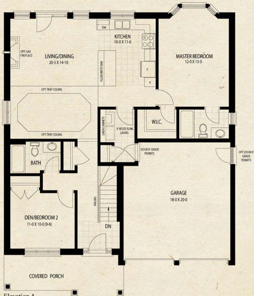
Elevation A Ground Floor Plan
