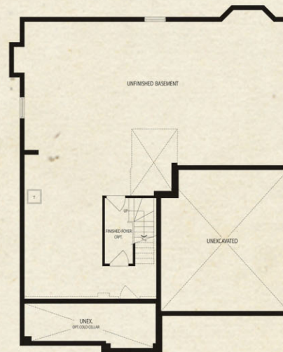
Elevation A Basement Floor Plan
