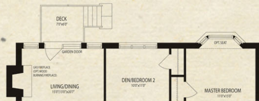
Elevation A & B Partial Ground Floor Plan WOD/WOB Condition
