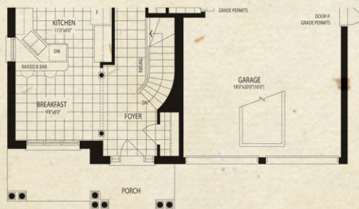
Elevation B Partial Ground Floor Plan
